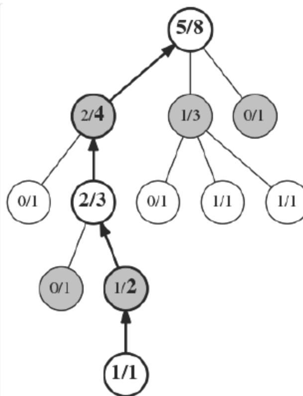
Back-Propagation
