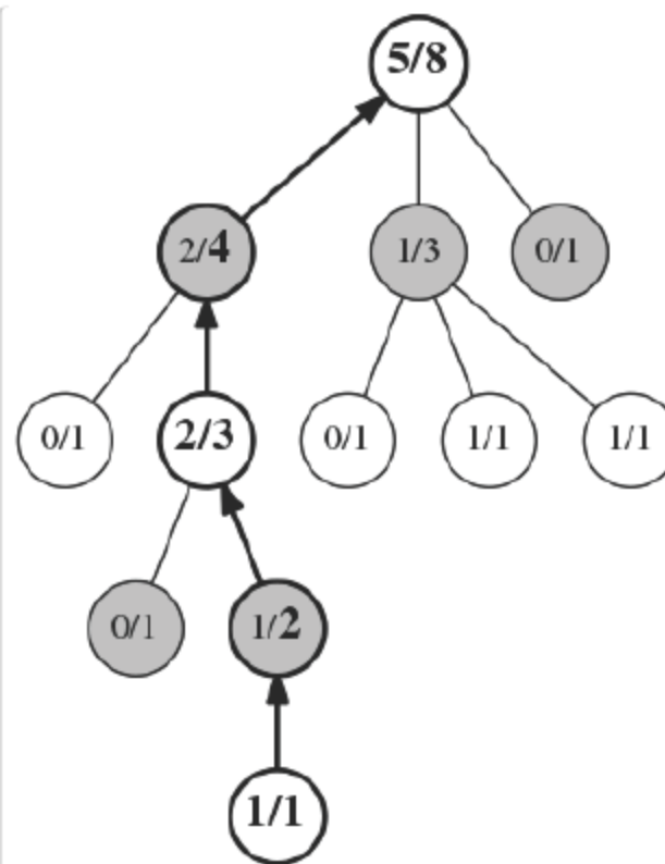
Back-Propagation
